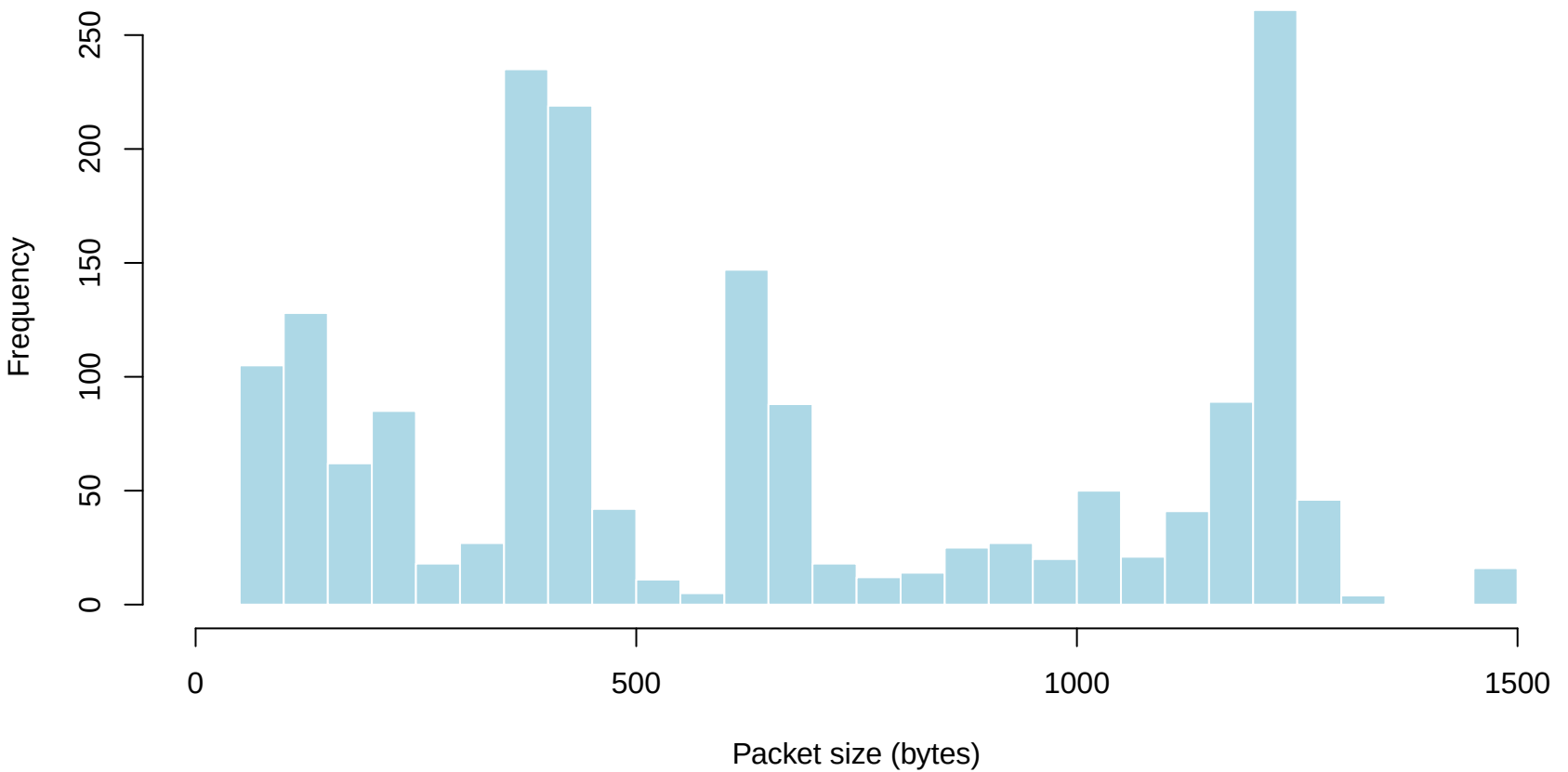
Packet sizes – normal state
